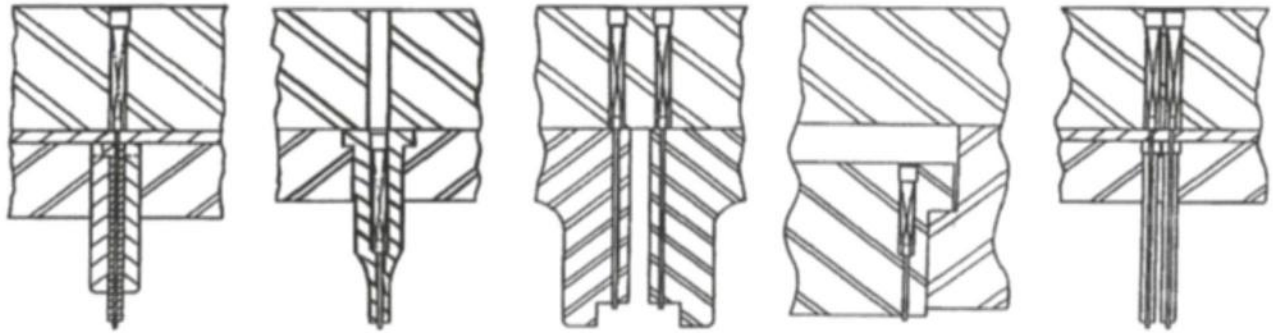
NARROW PUNCH IN SPLIT QUILL
